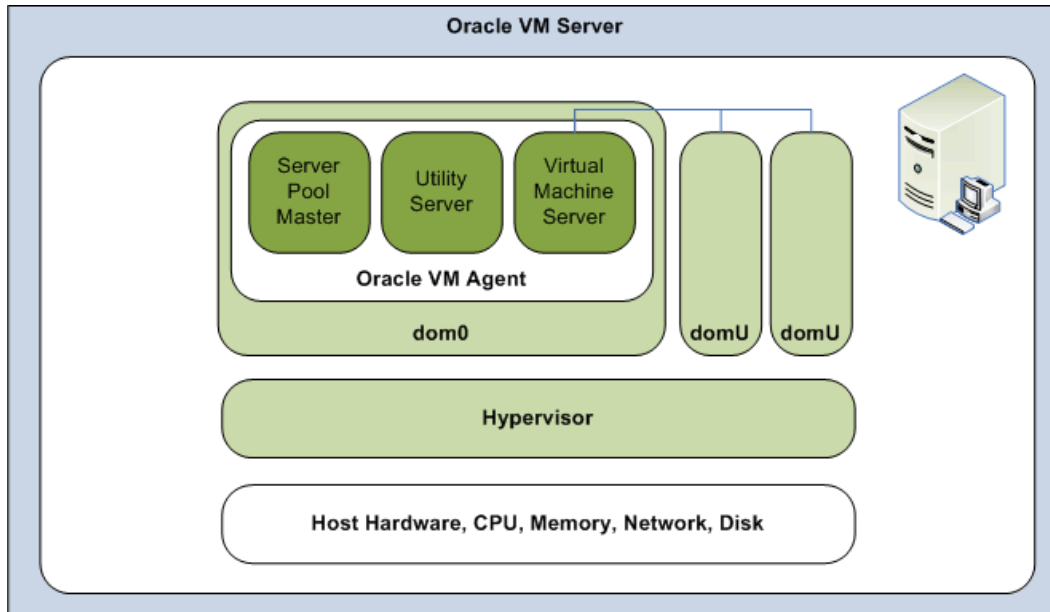
Figure 3: Oracle VM Server Architecture
